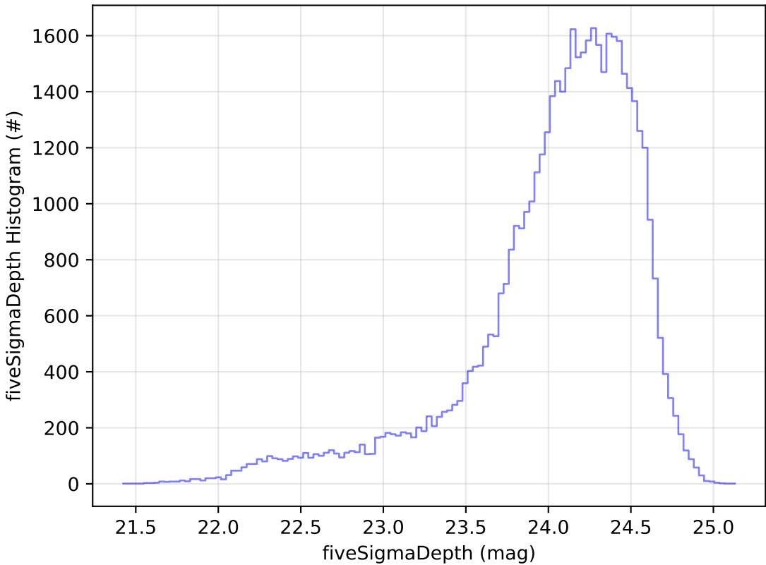
too_elab_r256_d2_griz_v3.4_10yrs Yr 1 r band: fiveSigmaDepth Histogram
