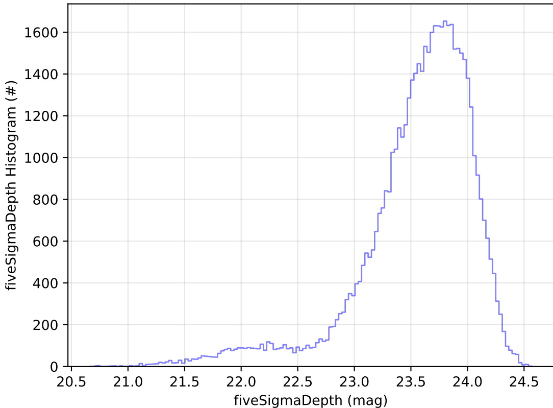
too_elab_r256_d2_griz_v3.4_10yrs Yr 1 i band: fiveSigmaDepth Histogram
