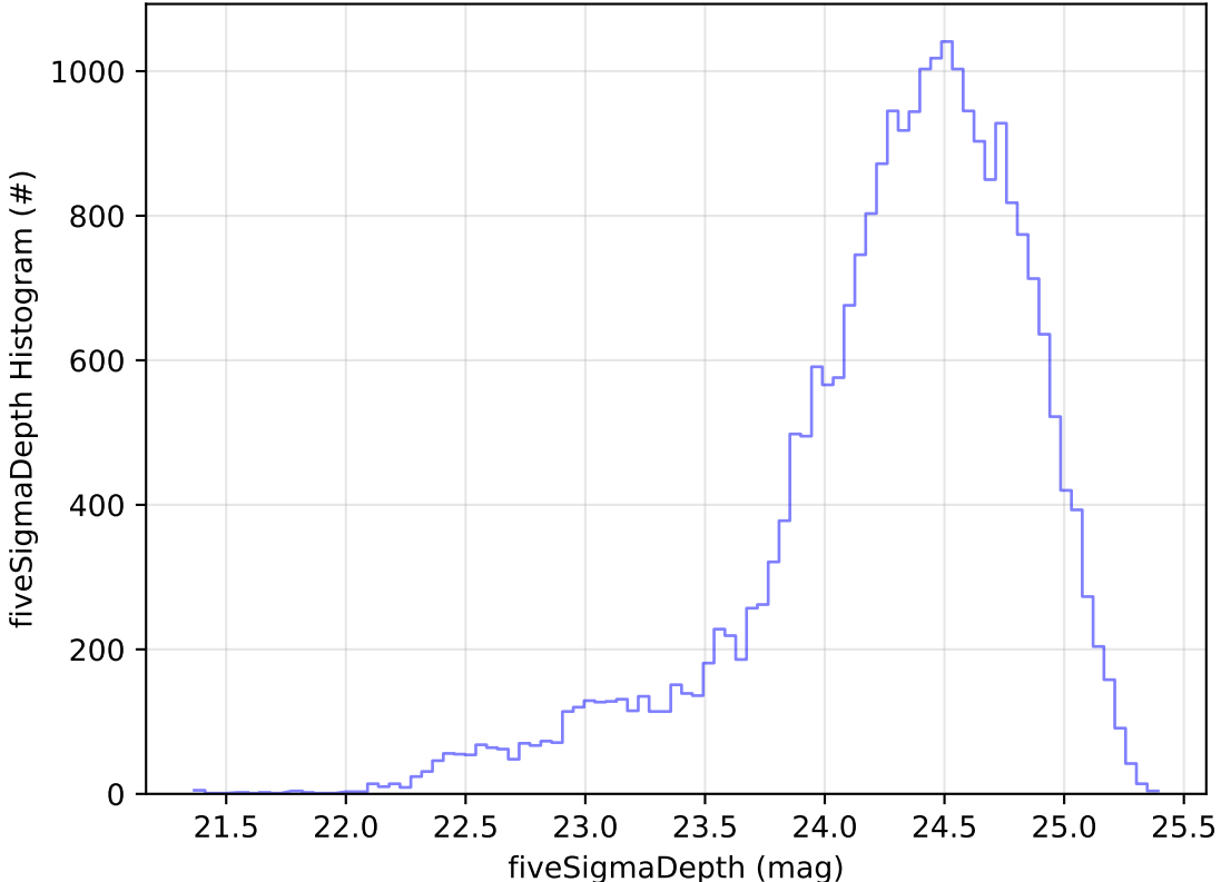
too_elab_r256_d2_griz_v3.4_10yrs Yr 1 g band: fiveSigmaDepth Histogram
