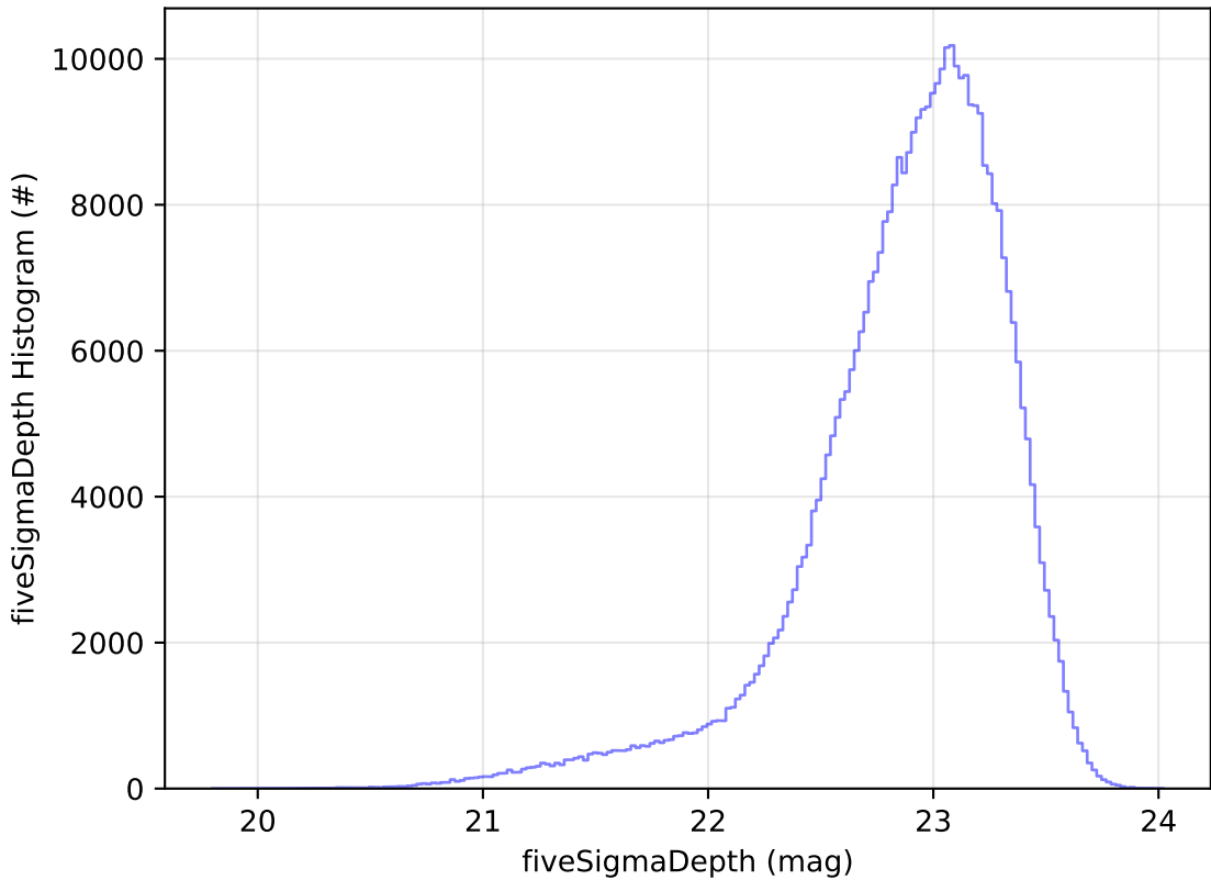
too_elab_r256_d2_griz_v3.4_10yrs WFD z band: fiveSigmaDepth Histogram
