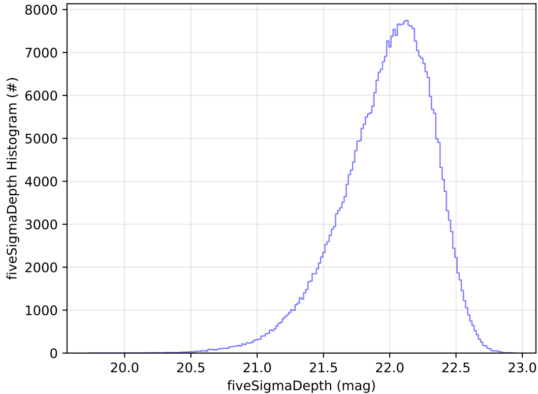
too_elab_r256_d2_griz_v3.4_10yrs WFD y band: fiveSigmaDepth Histogram
