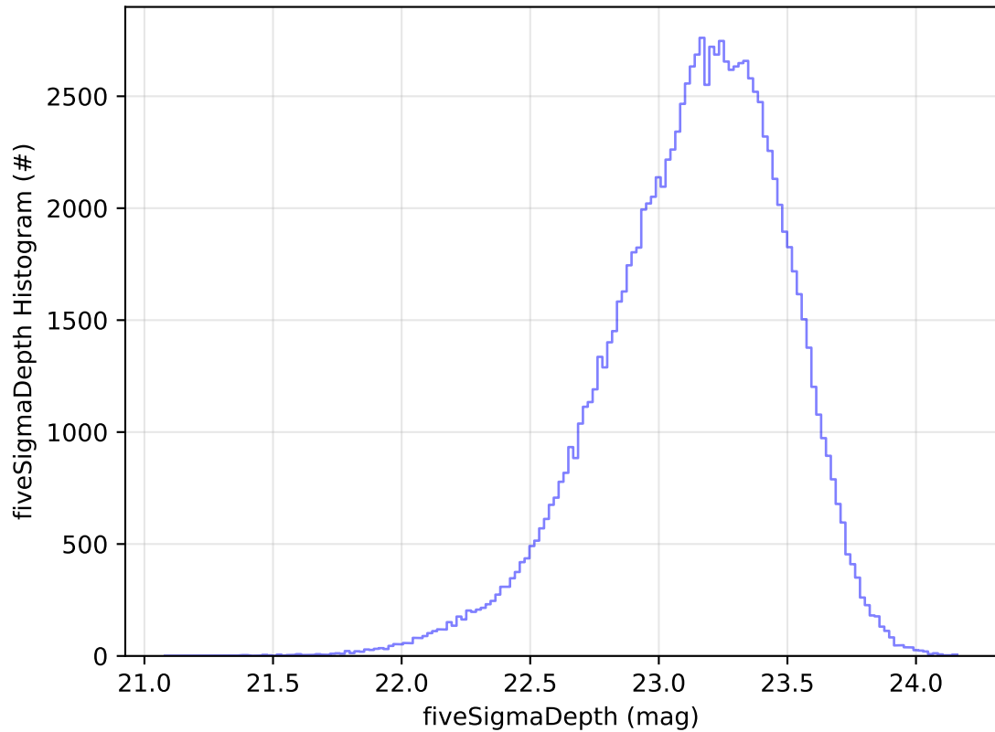
too_elab_r256_d2_griz_v3.4_10yrs WFD u band: fiveSigmaDepth Histogram
