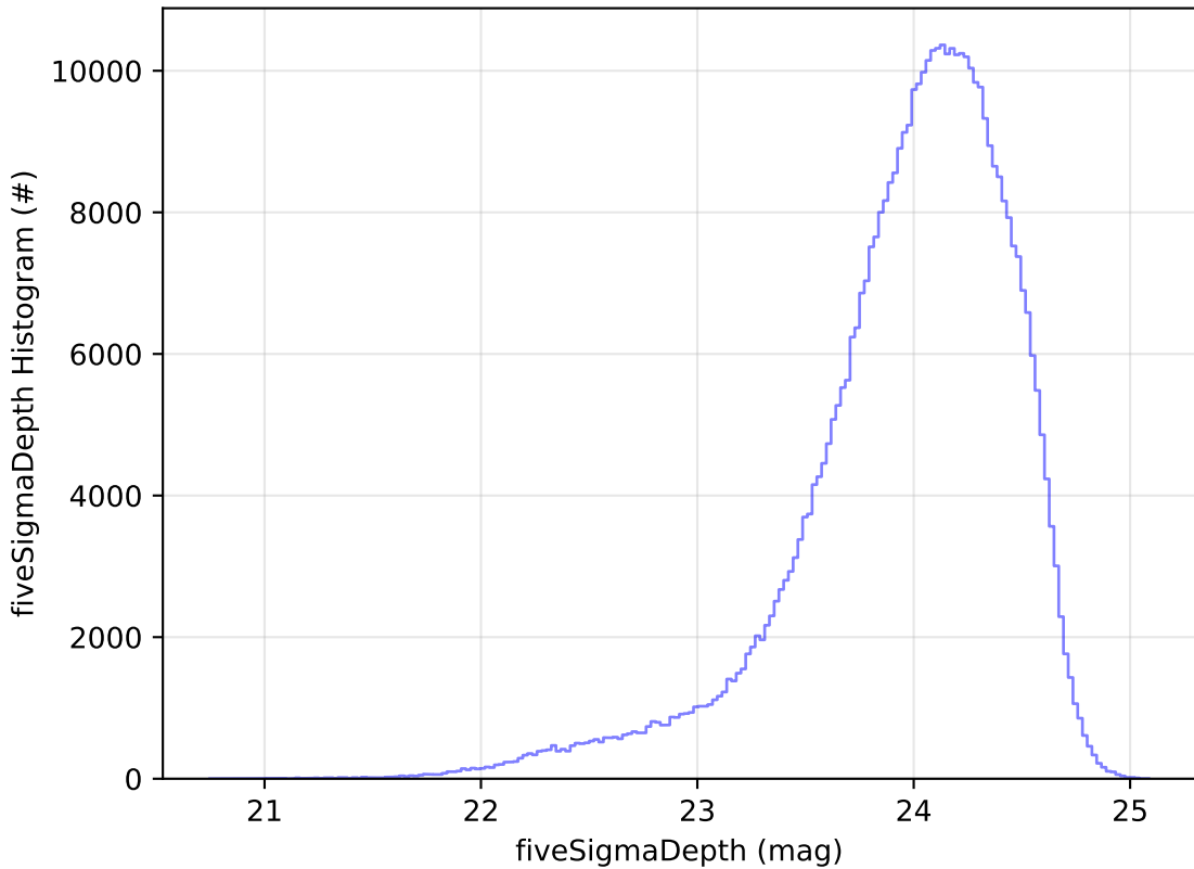
too_elab_r256_d2_griz_v3.4_10yrs WFD r band: fiveSigmaDepth Histogram
