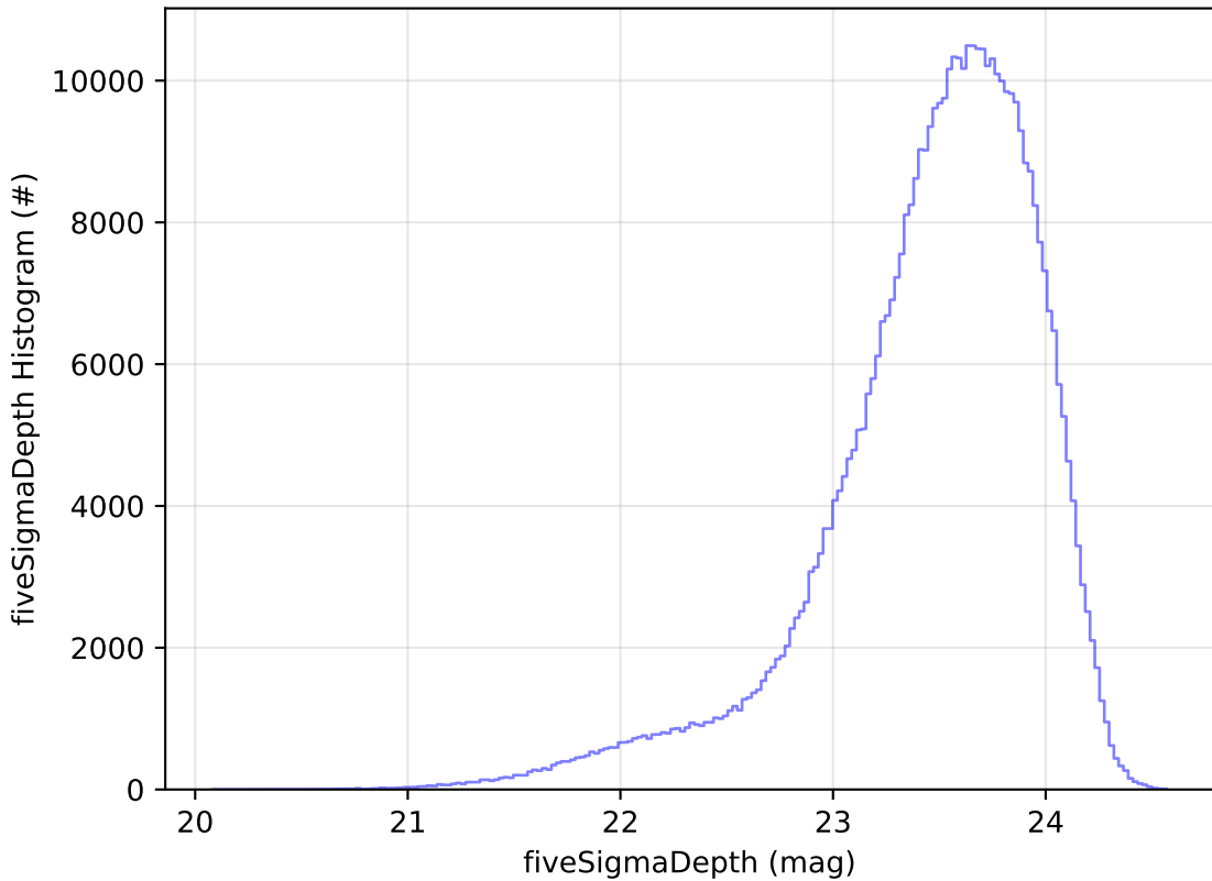
too_elab_r256_d2_griz_v3.4_10yrs WFD i band: fiveSigmaDepth Histogram
