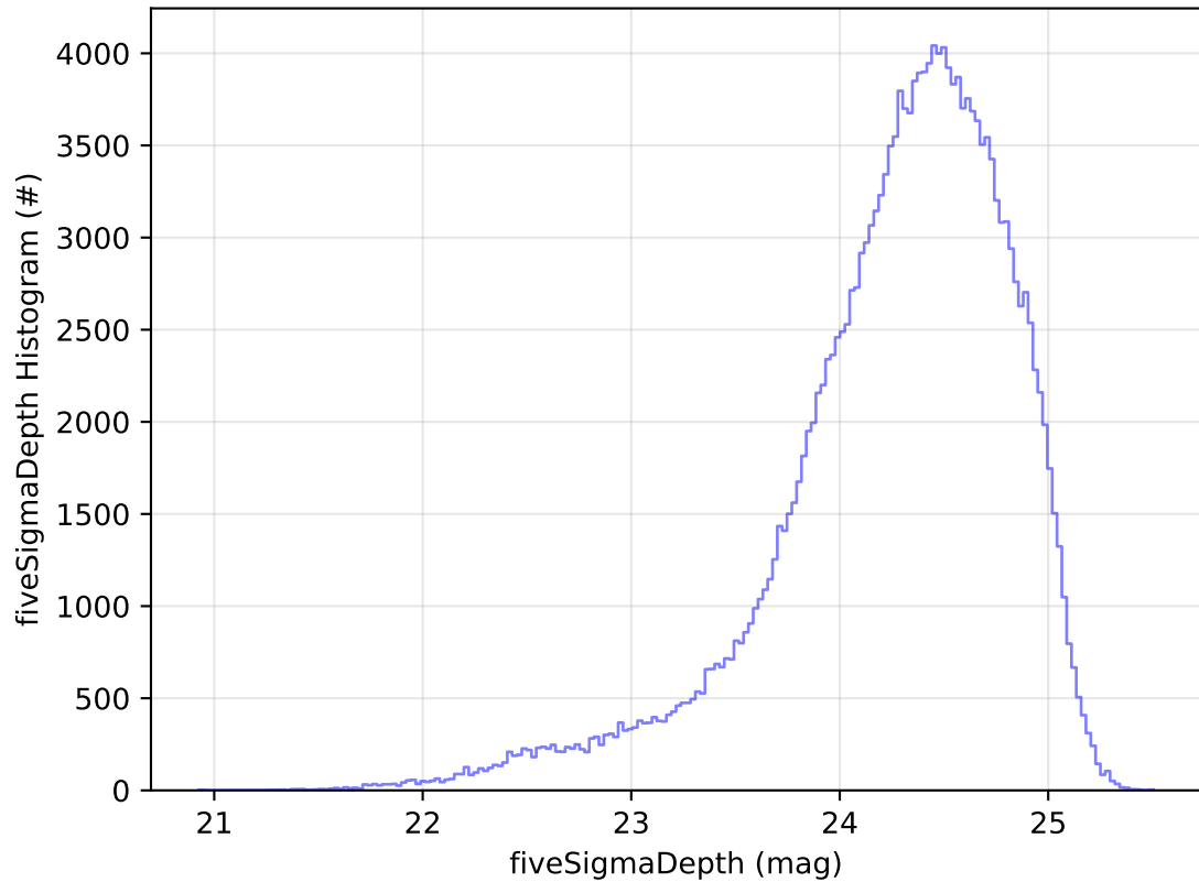
too_elab_r256_d2_griz_v3.4_10yrs WFD g band: fiveSigmaDepth Histogram
