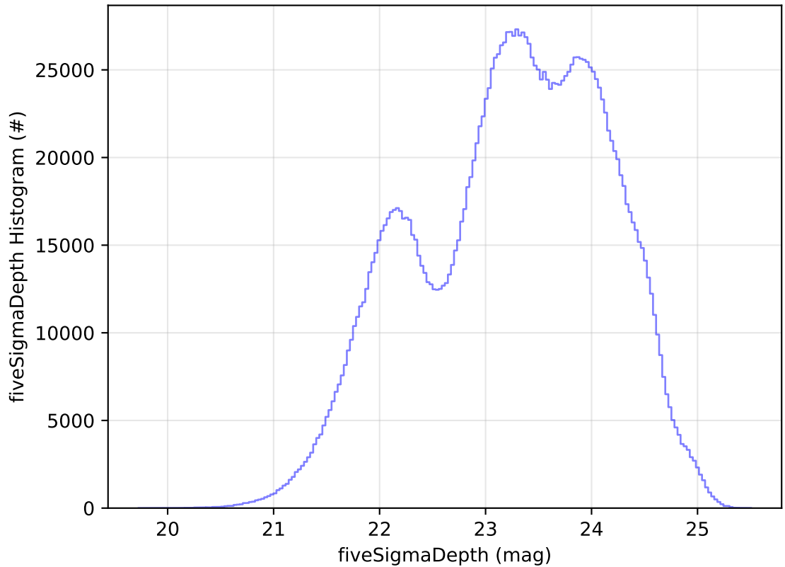
too_elab_r256_d2_griz_v3.4_10yrs WFD all bands: fiveSigmaDepth Histogram
