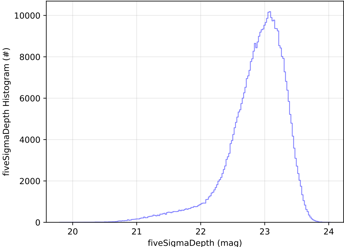
too_elab_r256_d2_griz_v3.4_10yrs All sky z band: fiveSigmaDepth Histogram
