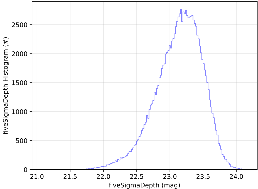
too_elab_r256_d2_griz_v3.4_10yrs All sky u band: fiveSigmaDepth Histogram
