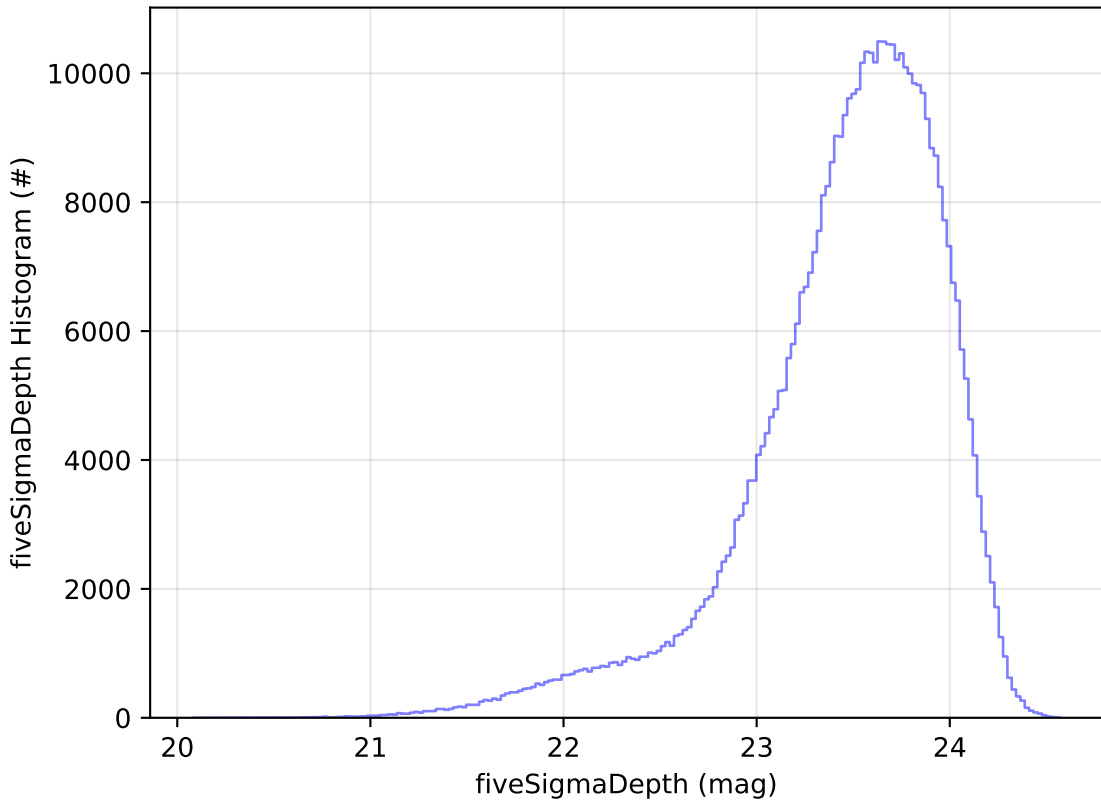
too_elab_r256_d2_griz_v3.4_10yrs All sky i band: fiveSigmaDepth Histogram
