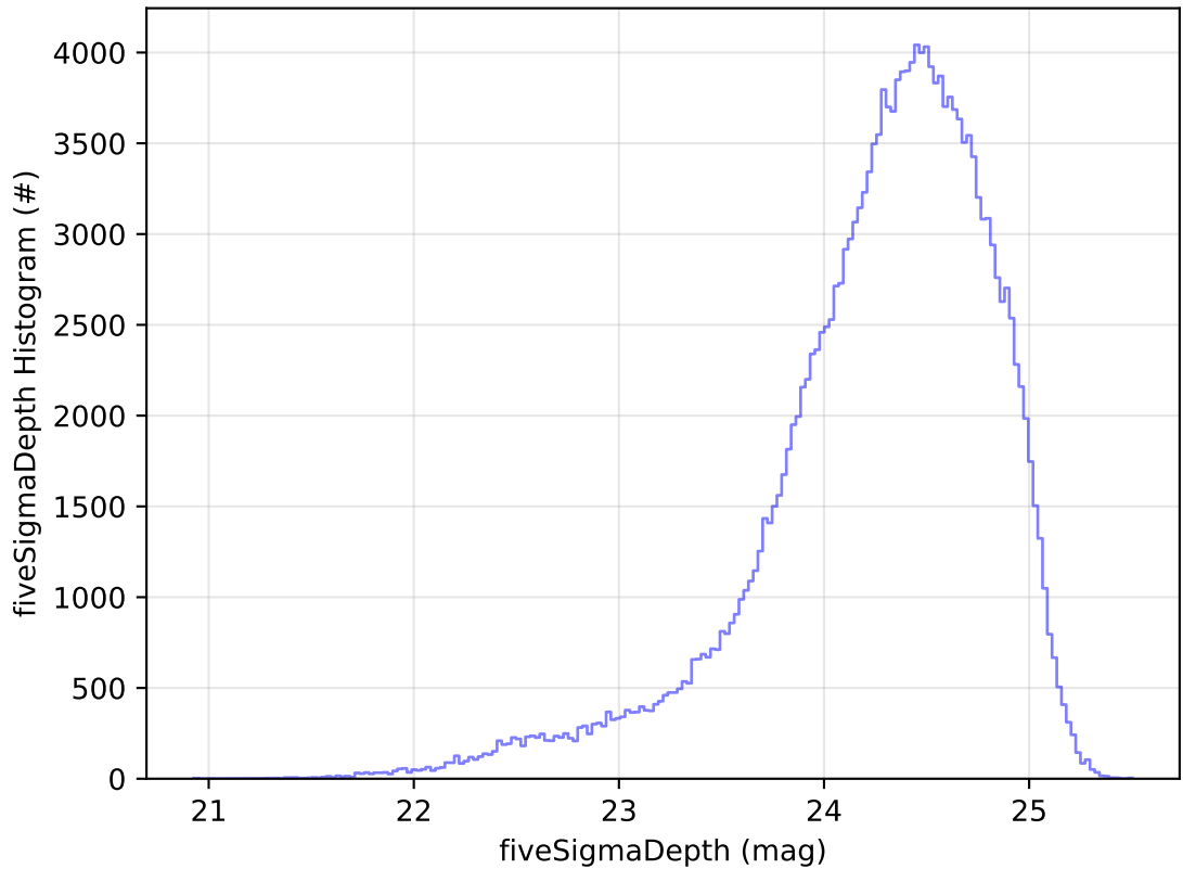
too_elab_r256_d2_griz_v3.4_10yrs All sky g band: fiveSigmaDepth Histogram
