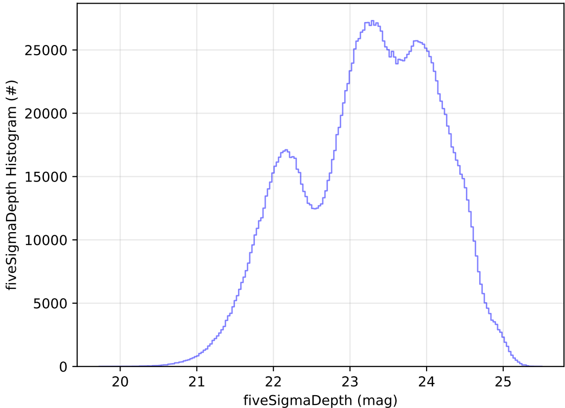
too_elab_r256_d2_griz_v3.4_10yrs All sky all bands: fiveSigmaDepth Histogram
