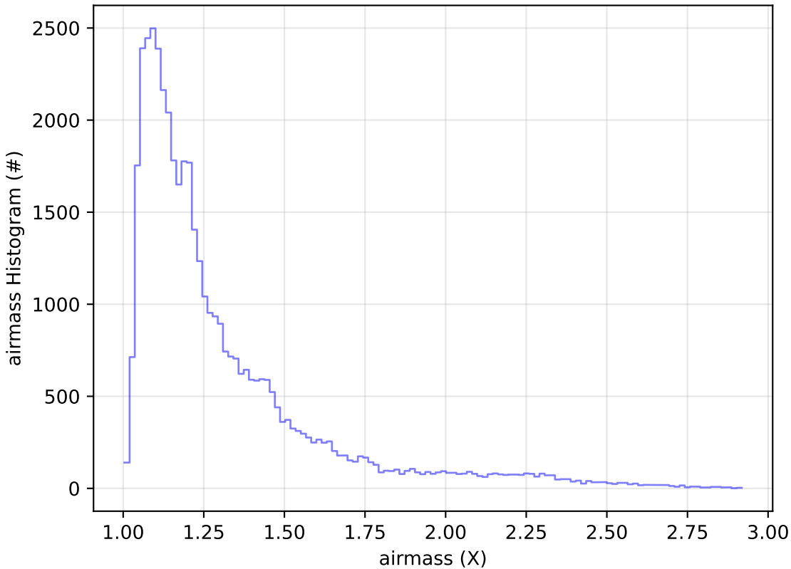
too_elab_r256_d2_griz_v3.4_10yrs Yr 1 z band: airmass Histogram
