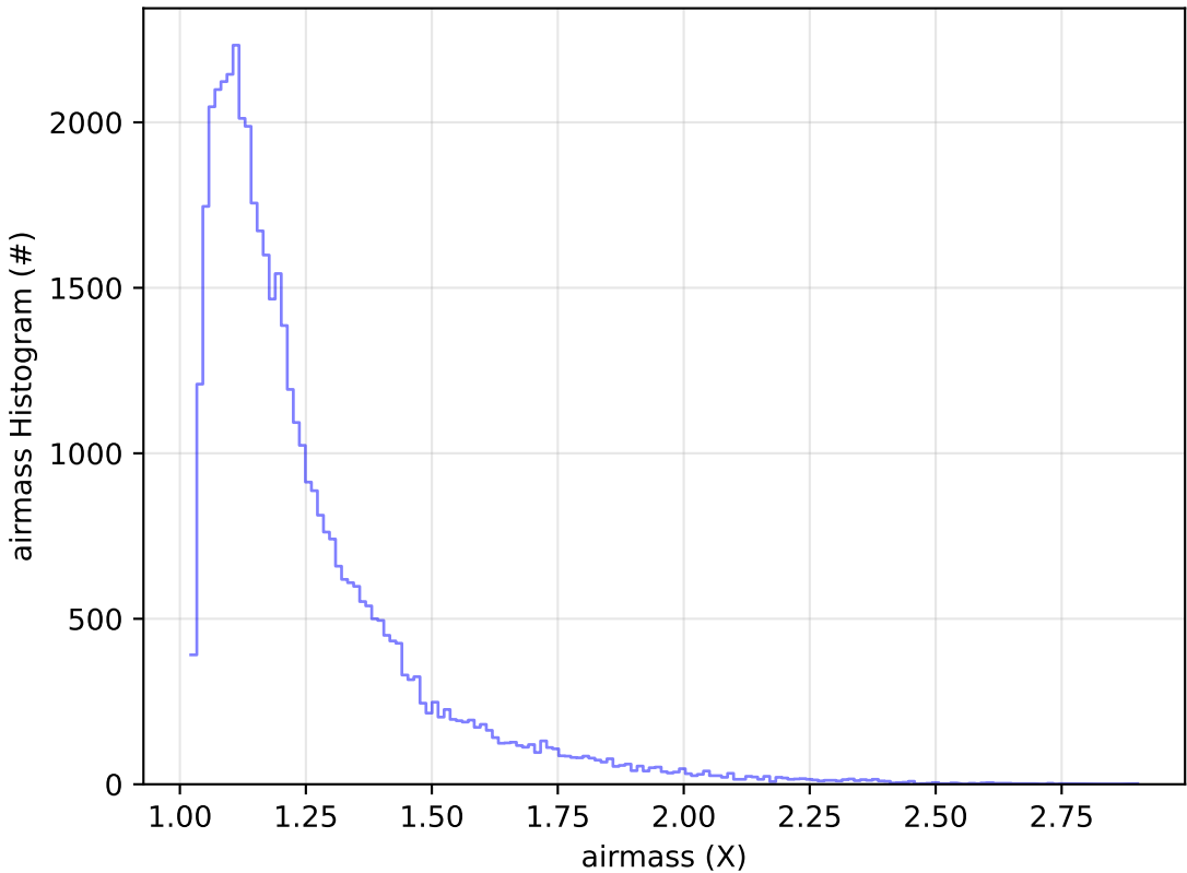
too_elab_r256_d2_griz_v3.4_10yrs Yr 1 y band: airmass Histogram
