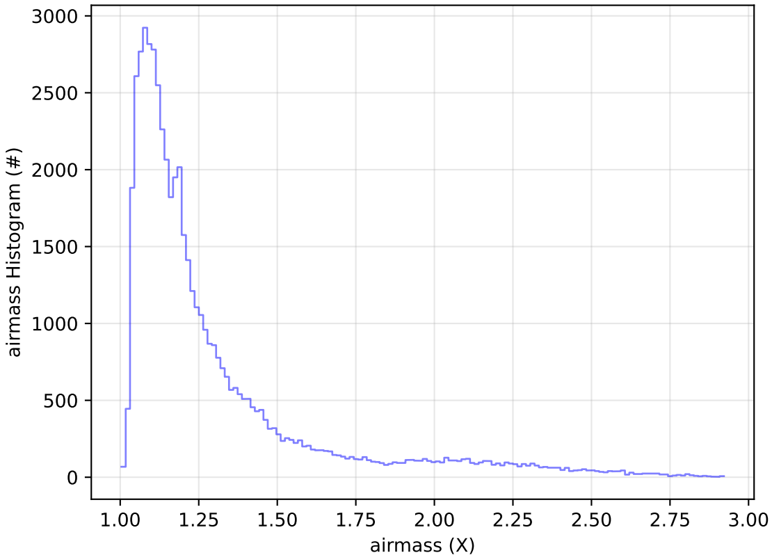
too_elab_r256_d2_griz_v3.4_10yrs Yr 1 i band: airmass Histogram
