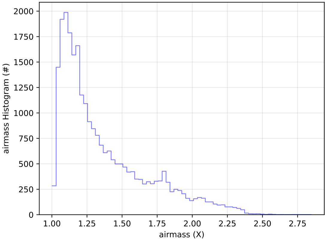
too_elab_r256_d2_griz_v3.4_10yrs Yr 1 g band: airmass Histogram
