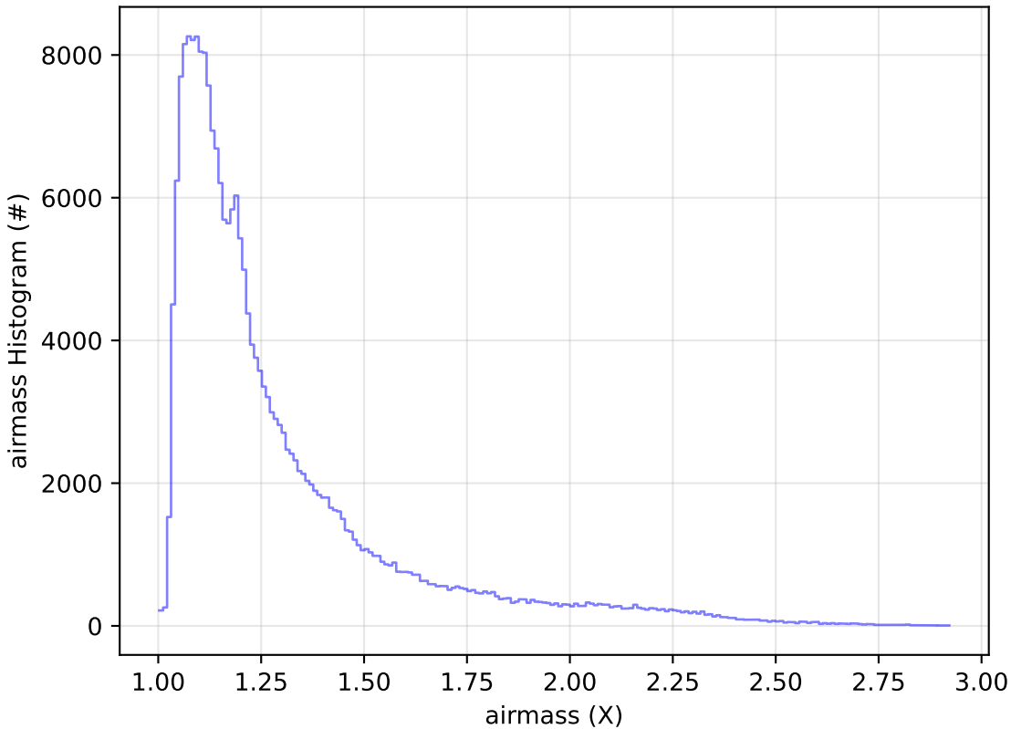
too_elab_r256_d2_griz_v3.4_10yrs Yr 1 all bands: airmass Histogram
