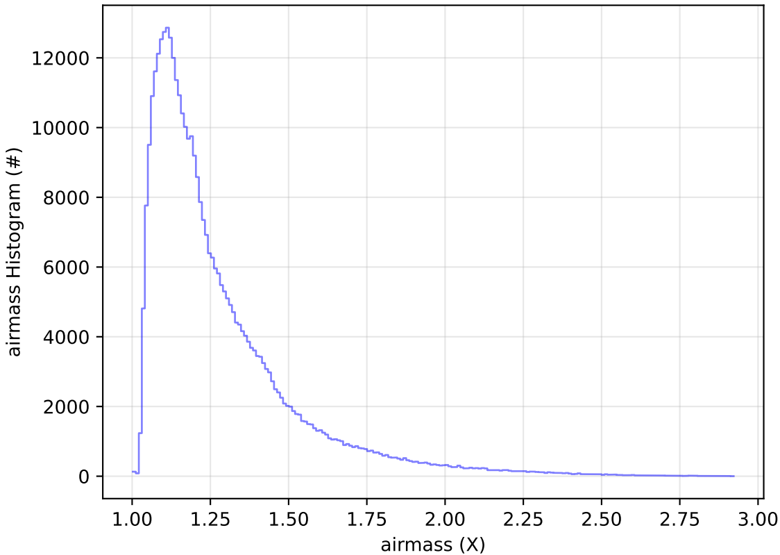
too_elab_r256_d2_griz_v3.4_10yrs WFD y band: airmass Histogram
