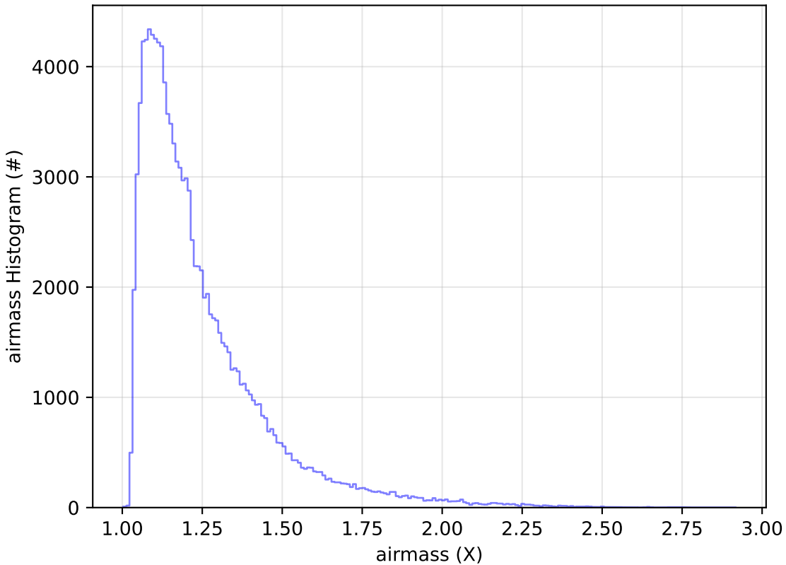
too_elab_r256_d2_griz_v3.4_10yrs WFD u band: airmass Histogram
