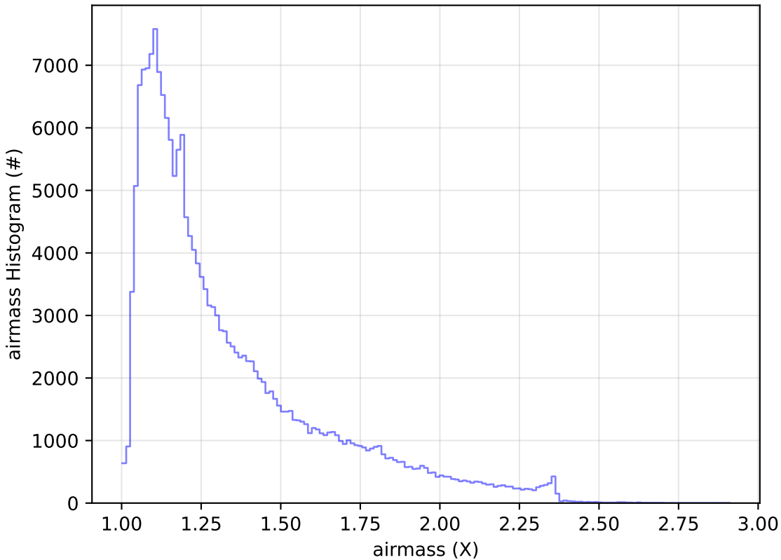
too_elab_r256_d2_griz_v3.4_10yrs WFD g band: airmass Histogram
