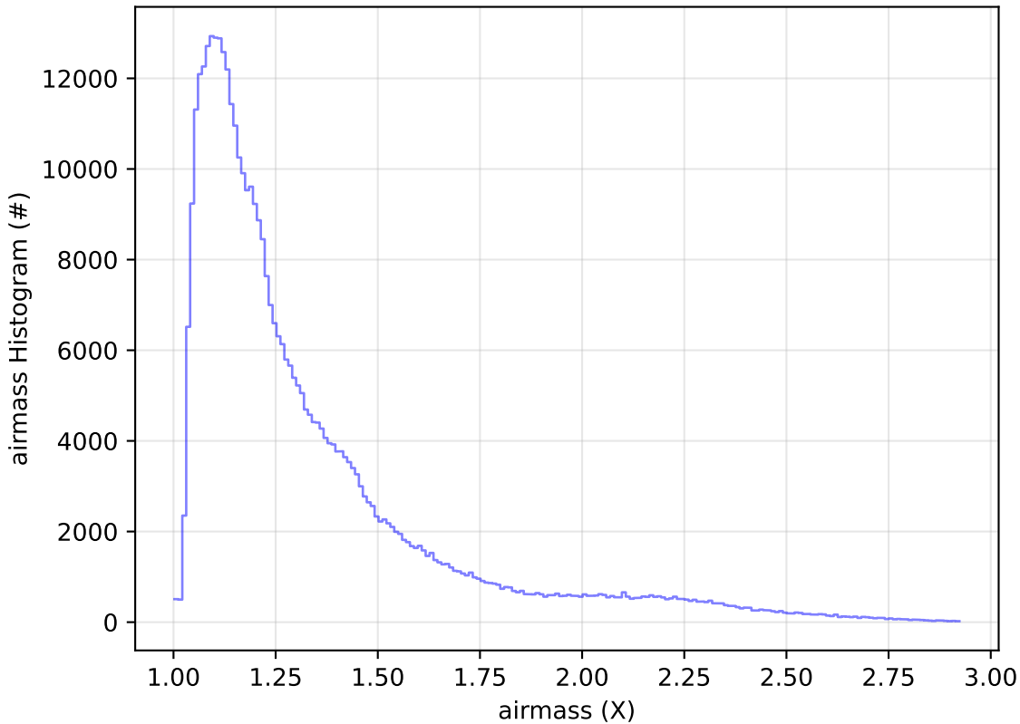
too_elab_r256_d2_griz_v3.4_10yrs All sky z band: airmass Histogram
