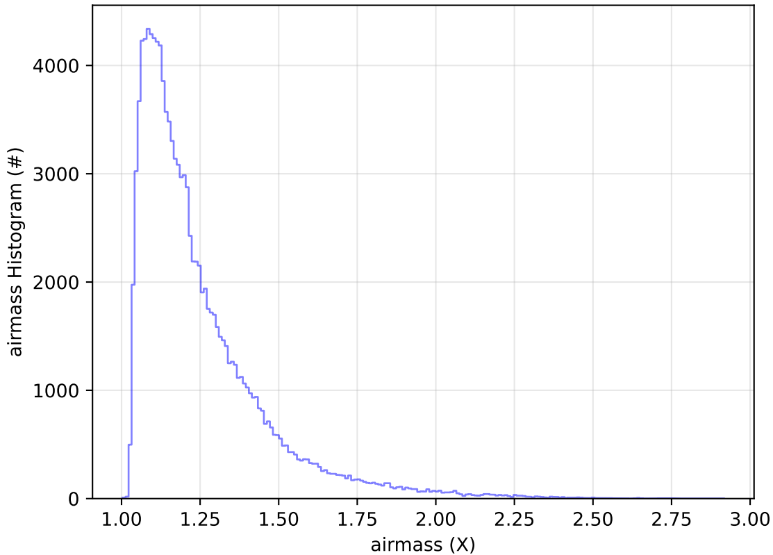
too_elab_r256_d2_griz_v3.4_10yrs All sky u band: airmass Histogram
