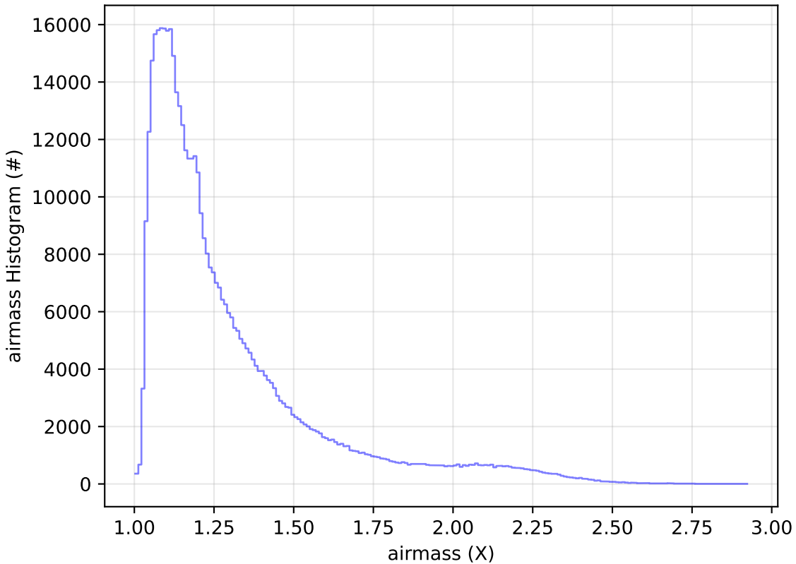
too_elab_r256_d2_griz_v3.4_10yrs All sky r band: airmass Histogram
