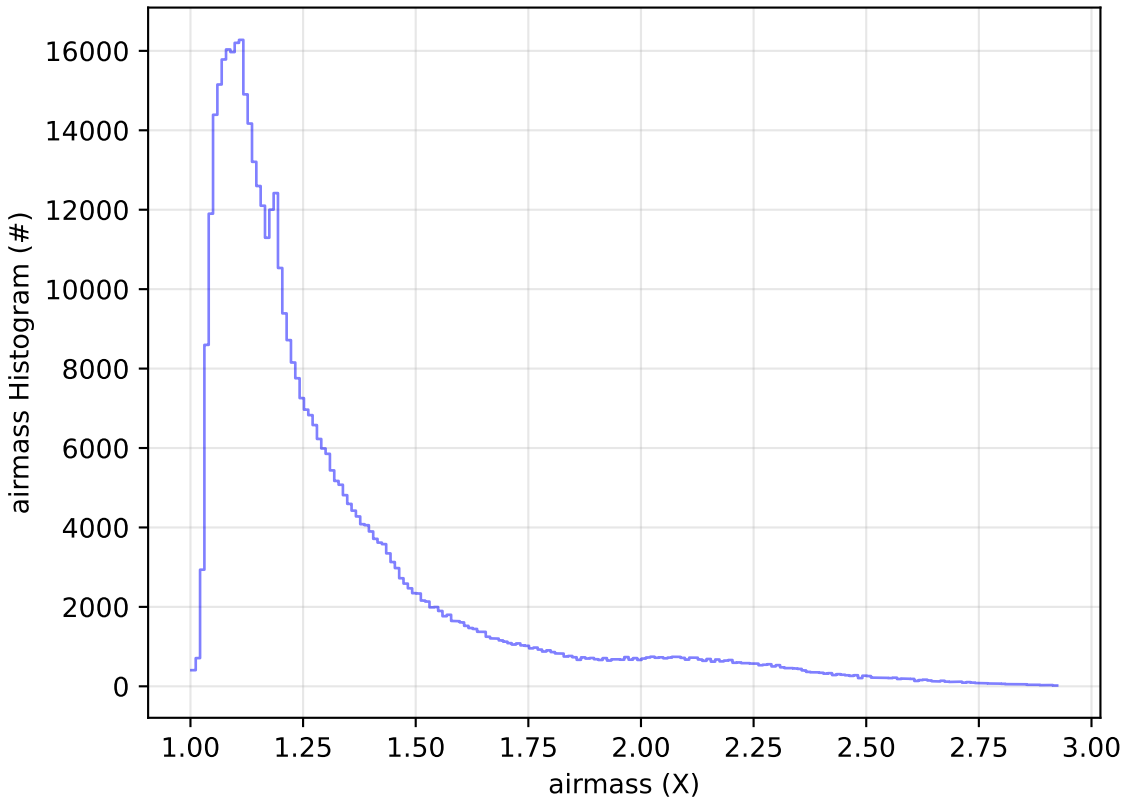
too_elab_r256_d2_griz_v3.4_10yrs All sky i band: airmass Histogram
