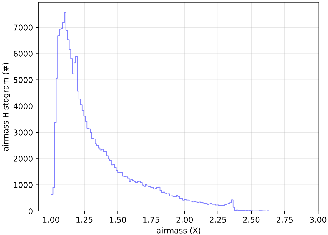
too_elab_r256_d2_griz_v3.4_10yrs All sky g band: airmass Histogram
