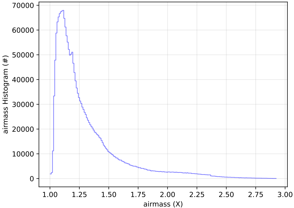
too_elab_r256_d2_griz_v3.4_10yrs All sky all bands: airmass Histogram
