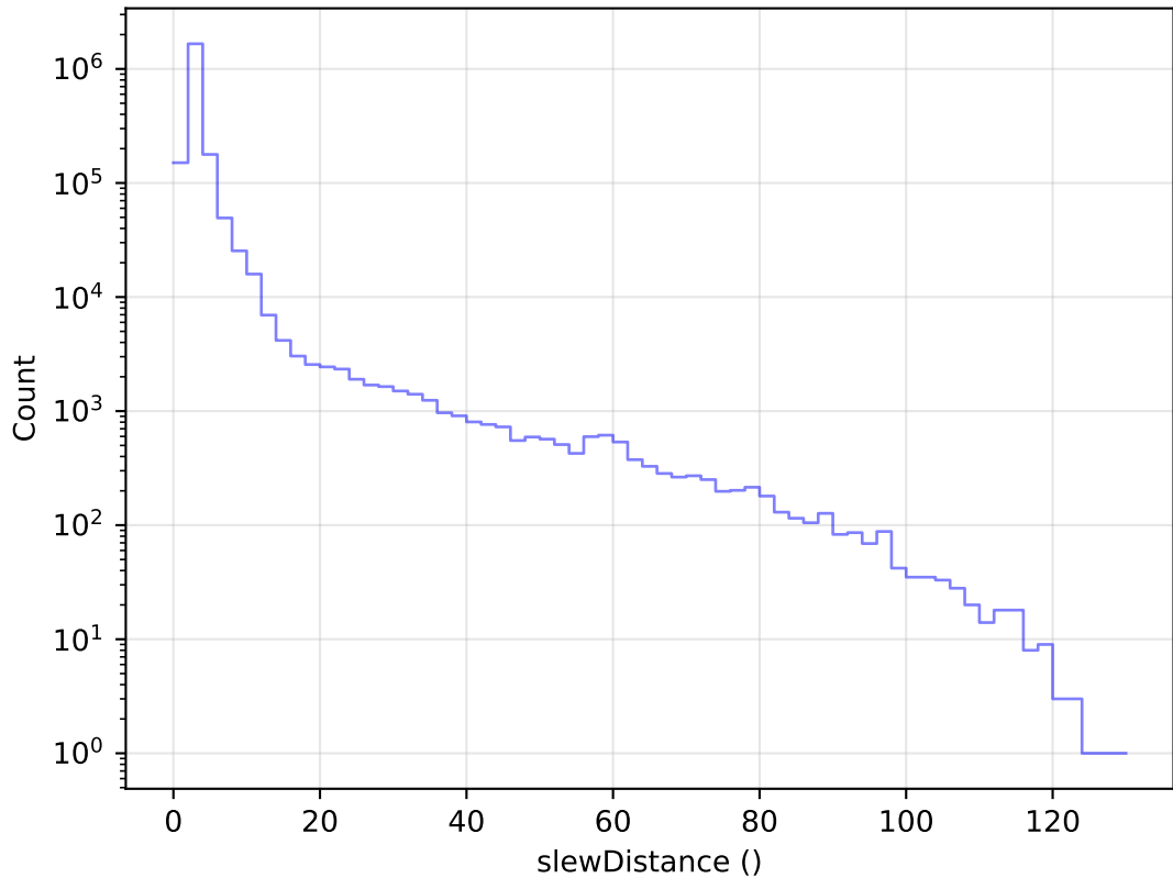
too_elab_r256_d2_griz_v3.4_10yrs All visits: Slew Distance Histogram
