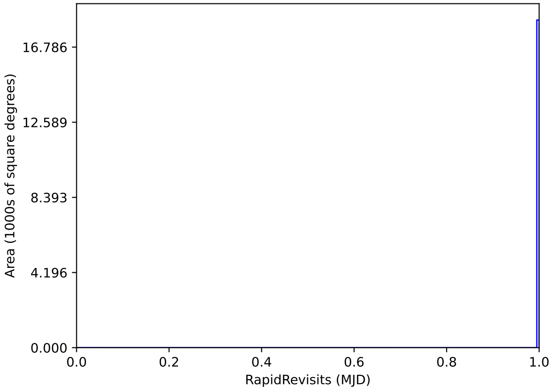
too_elab_r256_d2_griz_v3.4_10yrs WFD: RapidRevisits
