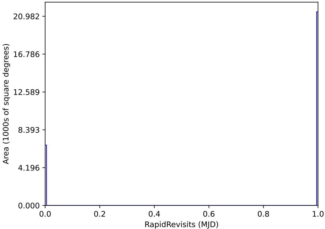
too_elab_r256_d2_griz_v3.4_10yrs All sky: RapidRevisits
