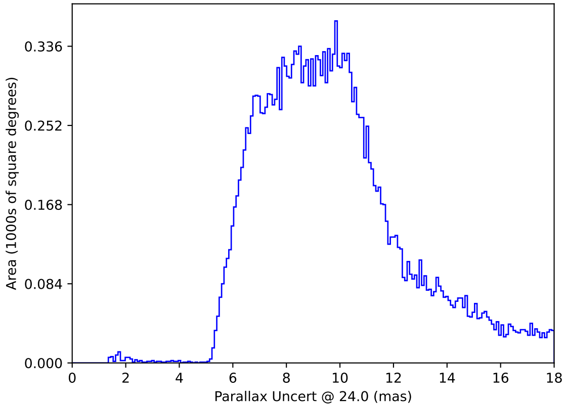
too_elab_r256_d2_griz_v3.4_10yrs All sky: Parallax Uncert @ 24.0
