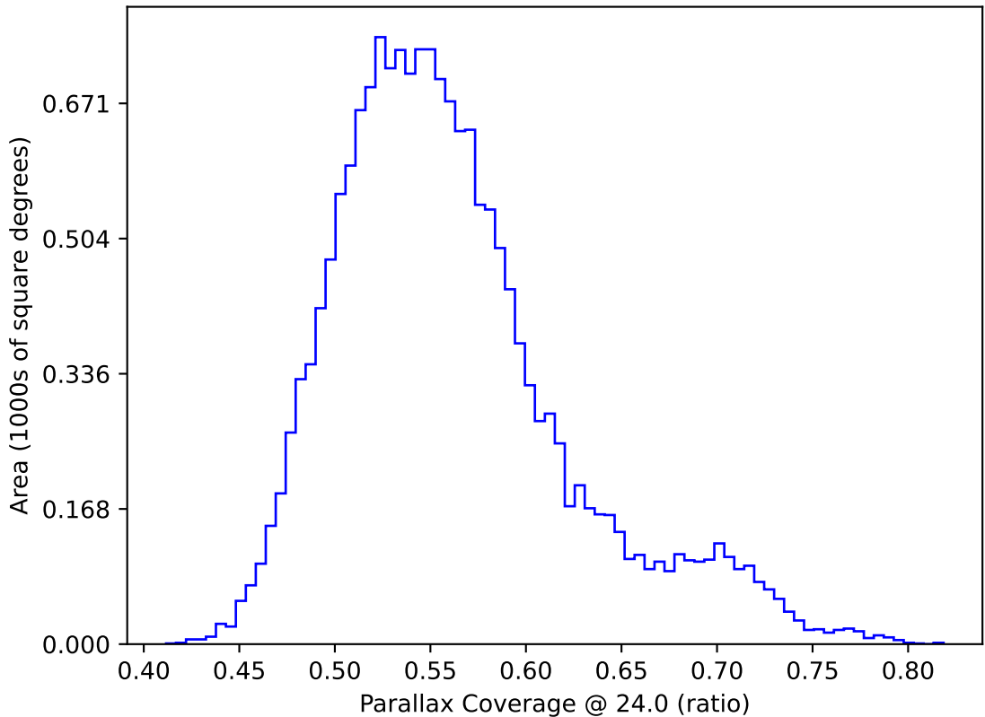
too_elab_r256_d2_griz_v3.4_10yrs WFD: Parallax Coverage @ 24.0
