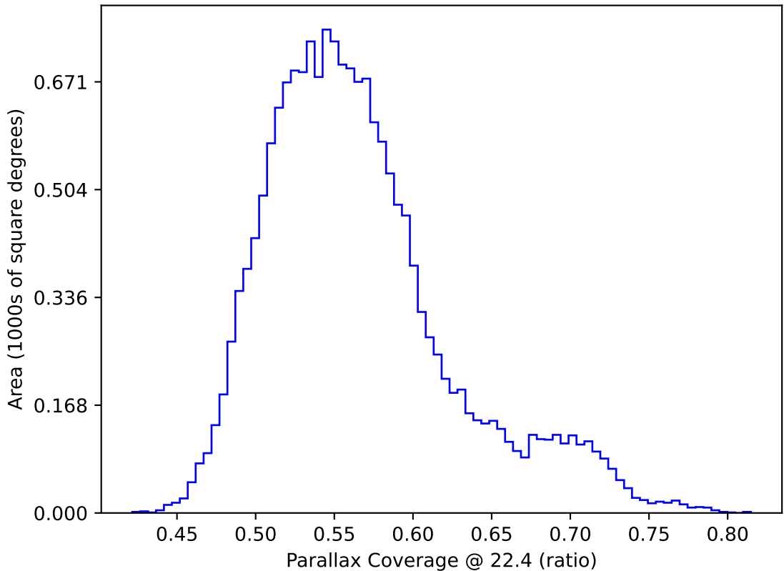
too_elab_r256_d2_griz_v3.4_10yrs WFD: Parallax Coverage @ 22.4
