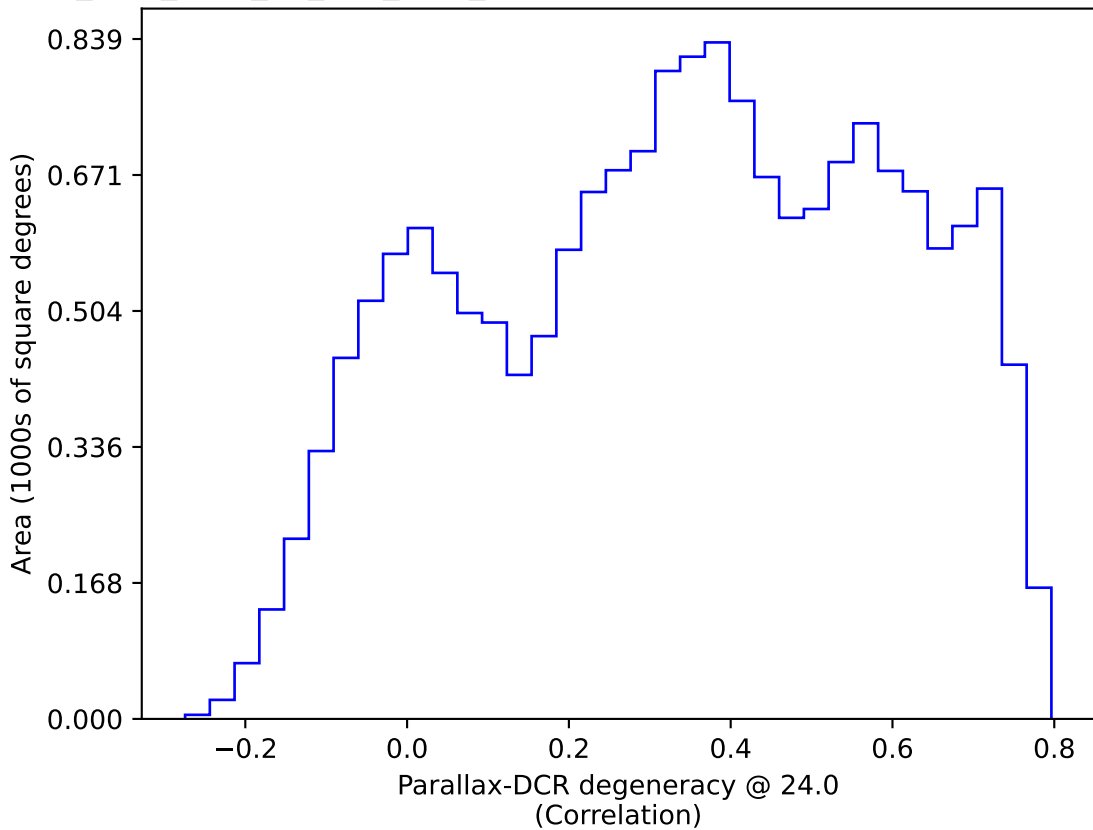
too_elab_r256_d2_griz_v3.4_10yrs WFD: Parallax-DCR degeneracy @ 24.0
