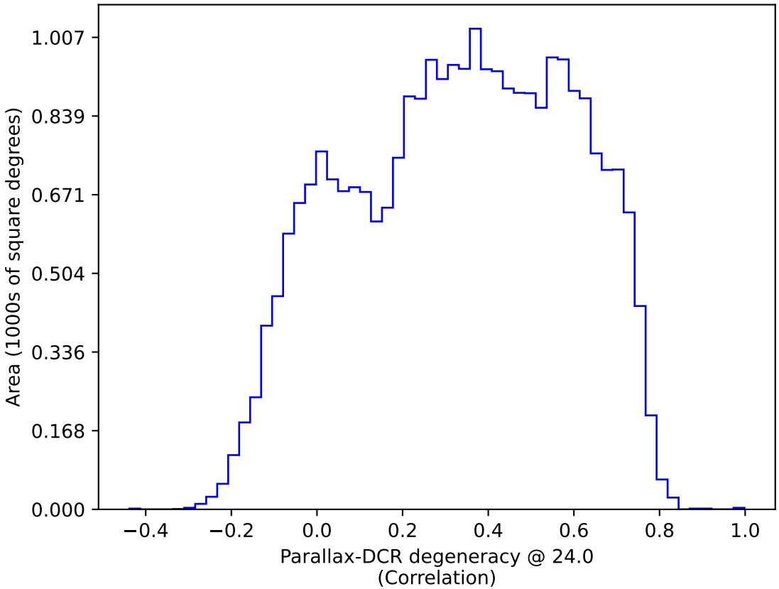
too_elab_r256_d2_griz_v3.4_10yrs All sky: Parallax-DCR degeneracy @ 24.0
