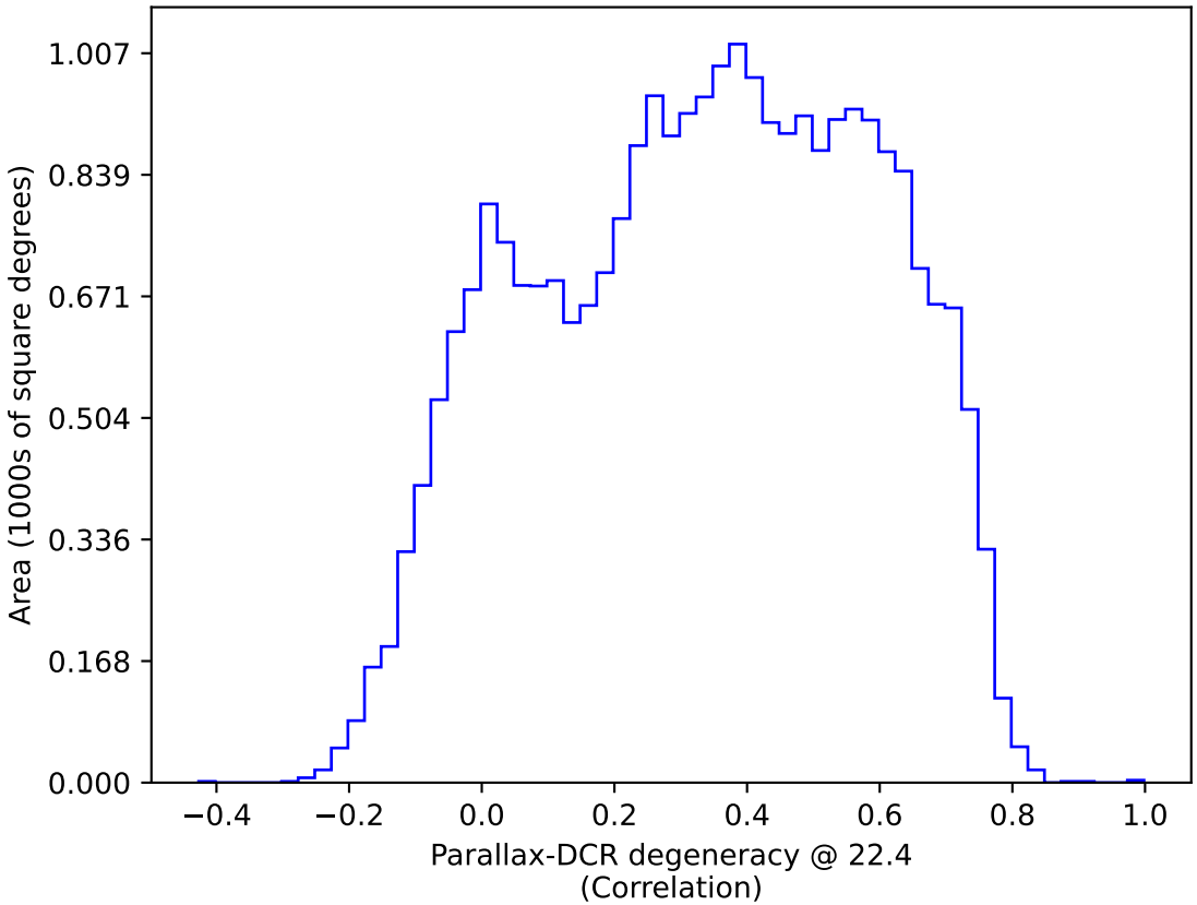
too_elab_r256_d2_griz_v3.4_10yrs All sky: Parallax-DCR degeneracy @ 22.4
