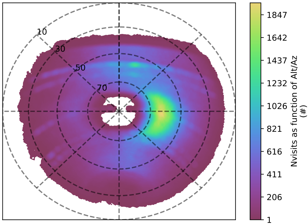
too_elab_r256_d2_griz_v3.4_10yrs y band: Nvisits as function of Alt/Az
