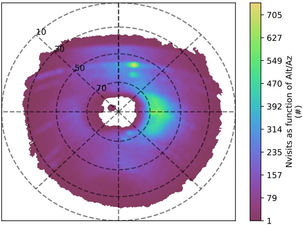
too_elab_r256_d2_griz_v3.4_10yrs u band: Nvisits as function of Alt/Az
