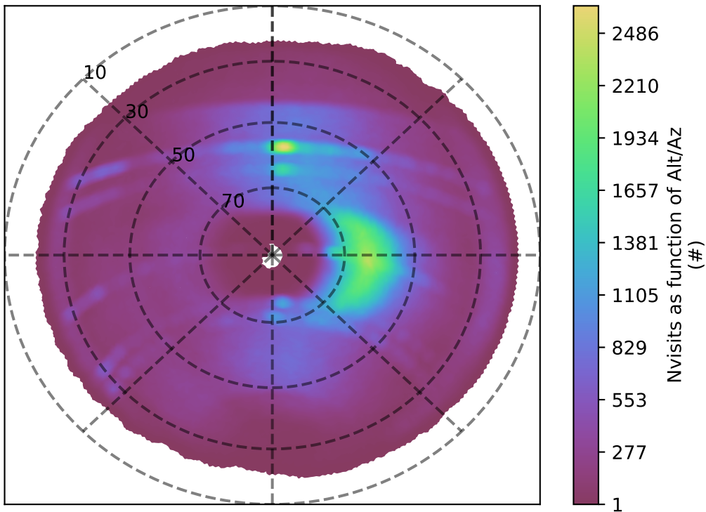
too_elab_r256_d2_griz_v3.4_10yrs i band: Nvisits as function of Alt/Az
