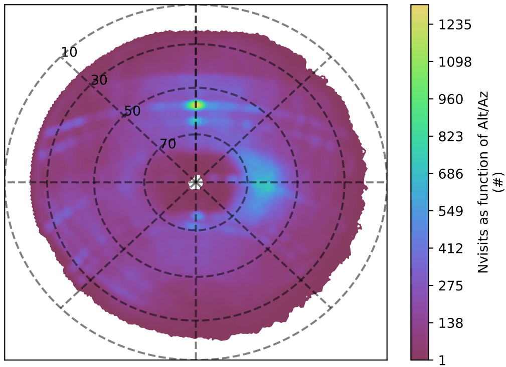
too_elab_r256_d2_griz_v3.4_10yrs g band: Nvisits as function of Alt/Az
