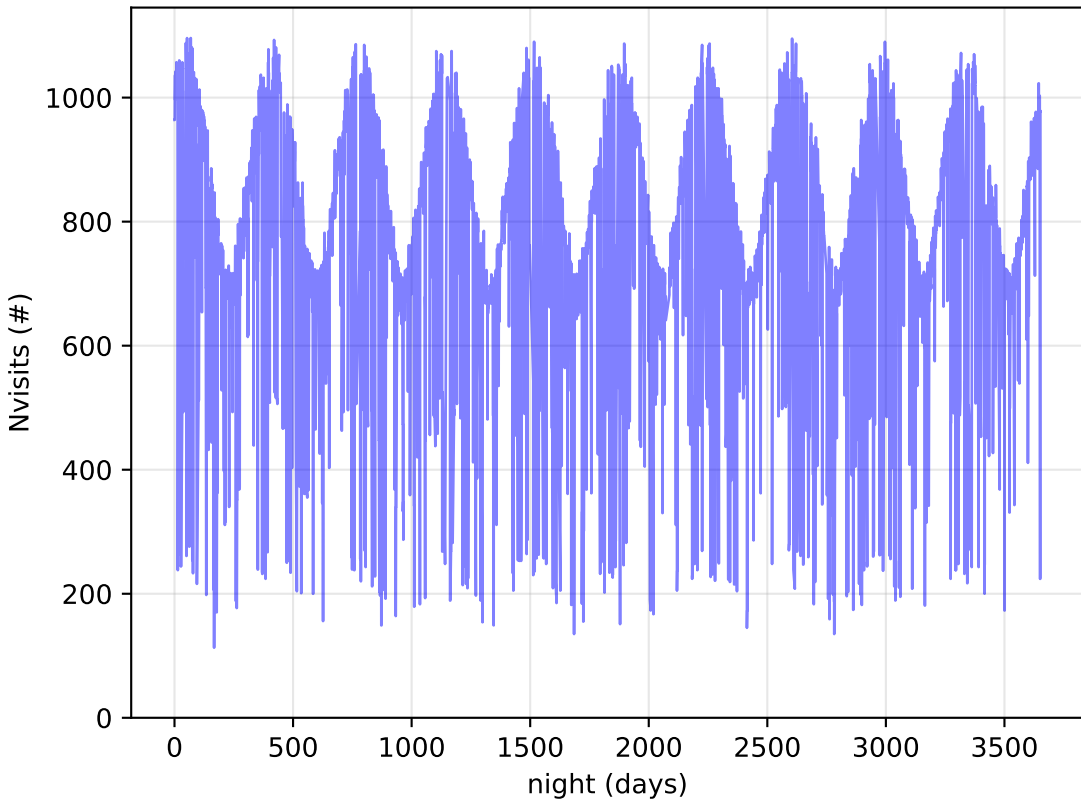
too_elab_r256_d2_griz_v3.4_10yrs All visits: Nvisits
