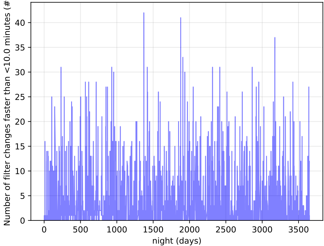
too_elab_r256_d2_griz_v3.4_10yrs Per Night: Number of filter changes faster than <10.0 minutes
