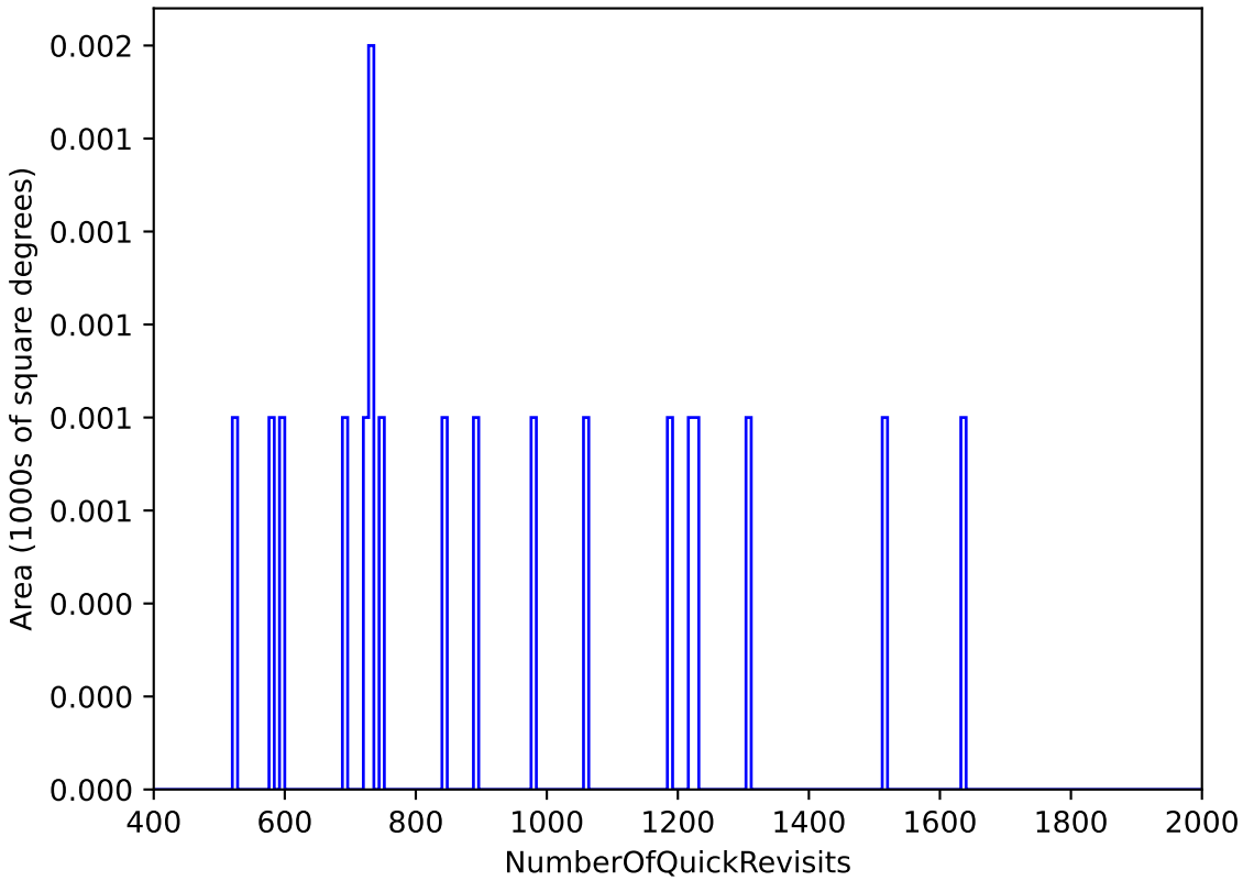
too_elab_r256_d2_griz_v3.4_10yrs WFD: NumberOfQuickRevisits
