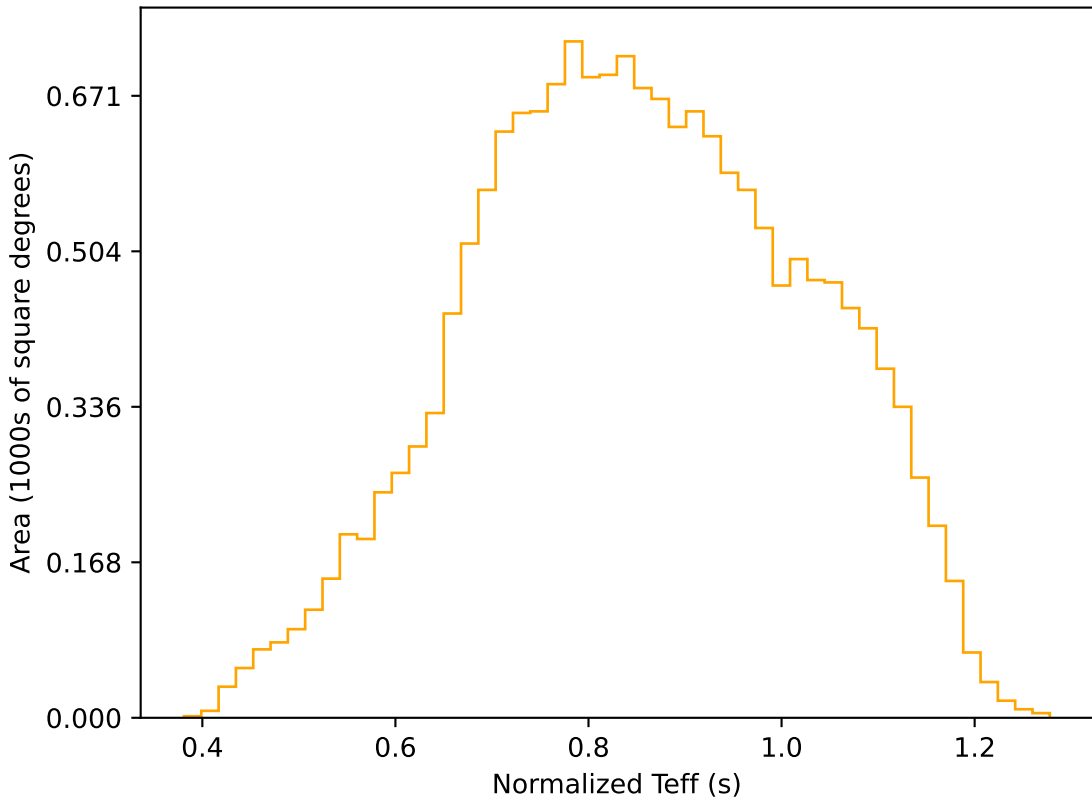
too_elab_r256_d2_griz_v3.4_10yrs WFD r band: Normalized Teff
