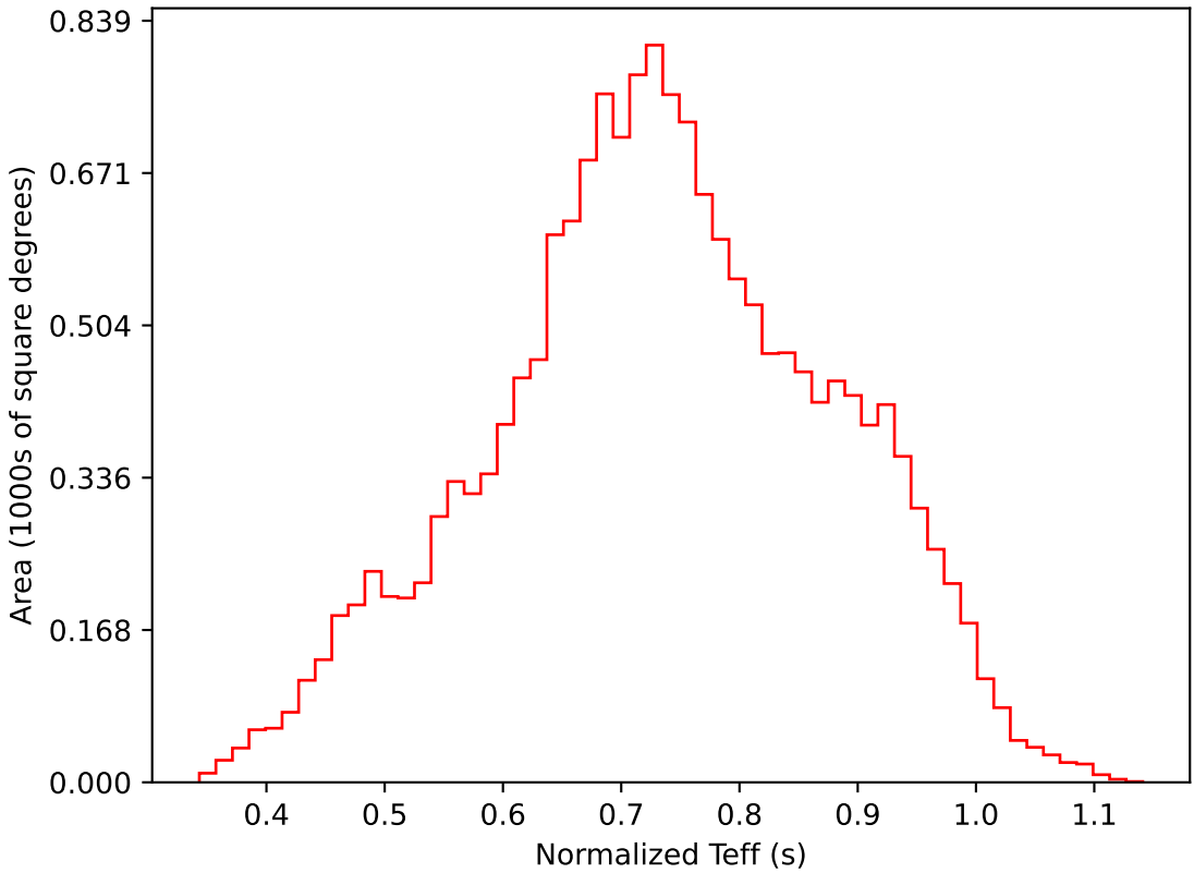
too_elab_r256_d2_griz_v3.4_10yrs WFD i band: Normalized Teff
