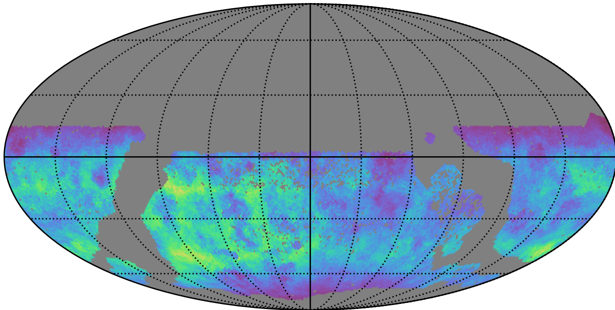
too_elab_r256_d2_griz_v3.4_10yrs WFD g band: Normalized Teff
