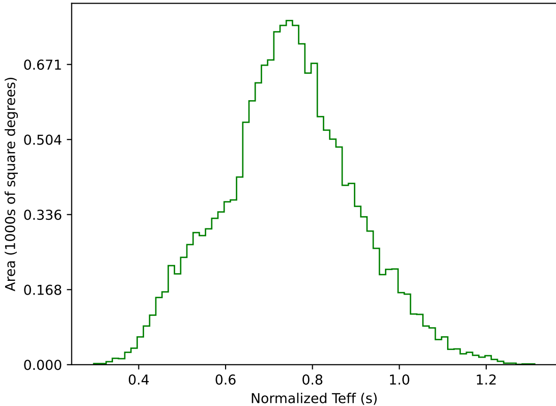
too_elab_r256_d2_griz_v3.4_10yrs WFD g band: Normalized Teff
