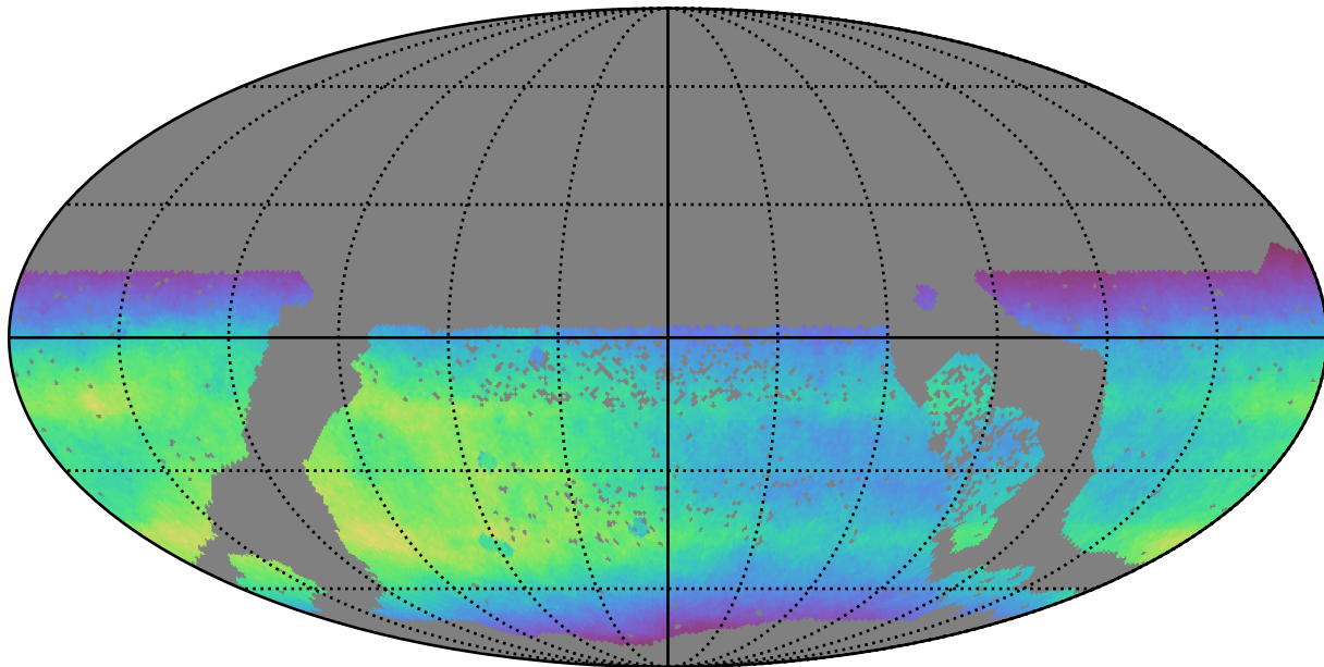
too_elab_r256_d2_griz_v3.4_10yrs WFD all bands: Normalized Teff
